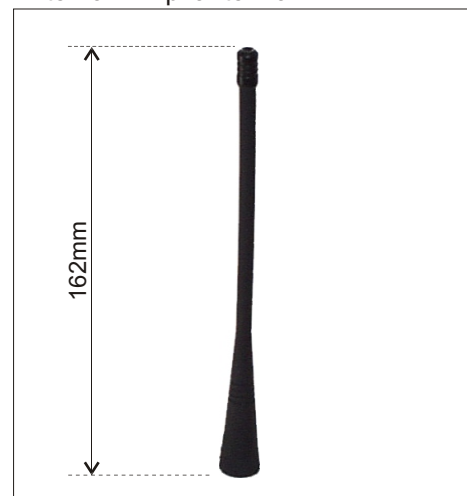
External 'whip' antenna
